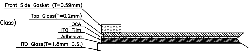
DETAIL B
