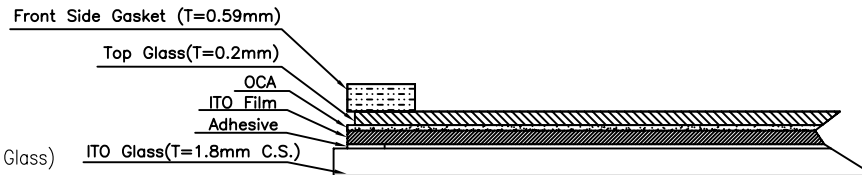
DETAIL A
